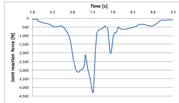
Fig. 3: Joint reaction forces directly into the cup. Positive values are instable.
